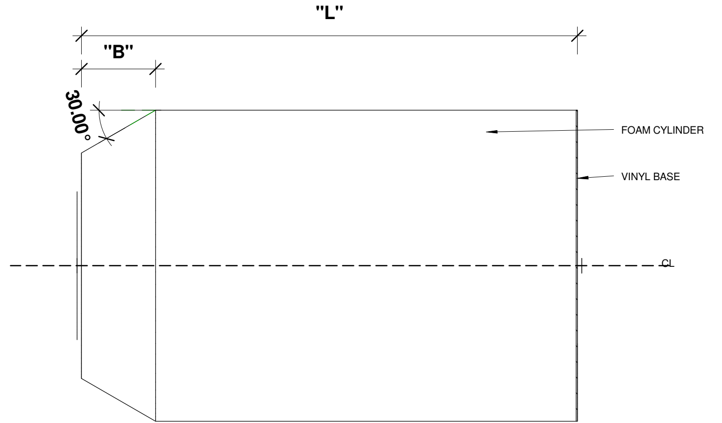
SIDE VIEW TYPE 01
